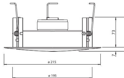
unit : mm Side view
